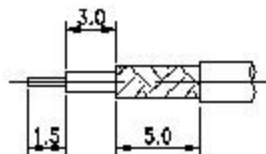
STRIPPING DIMENSION
